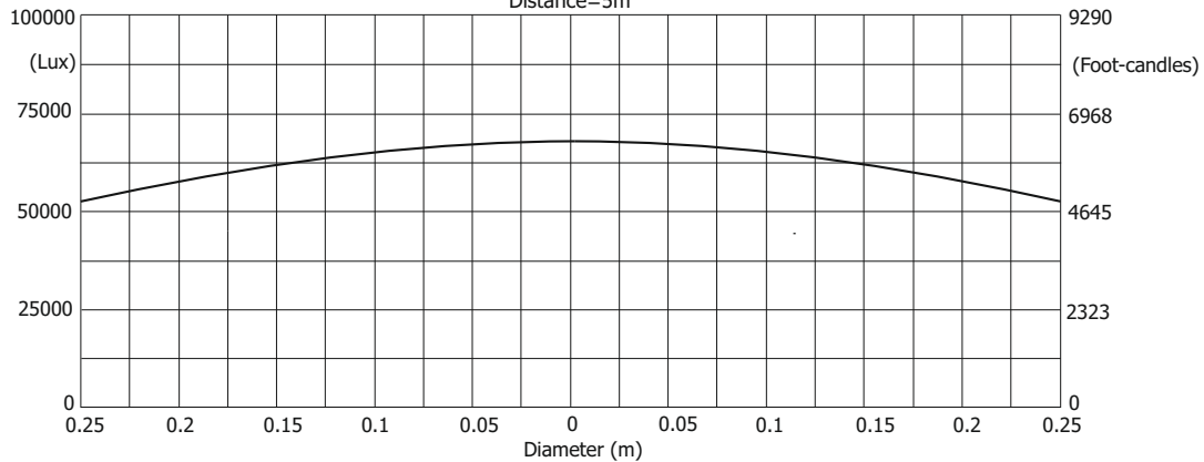
Illuminance distribution
