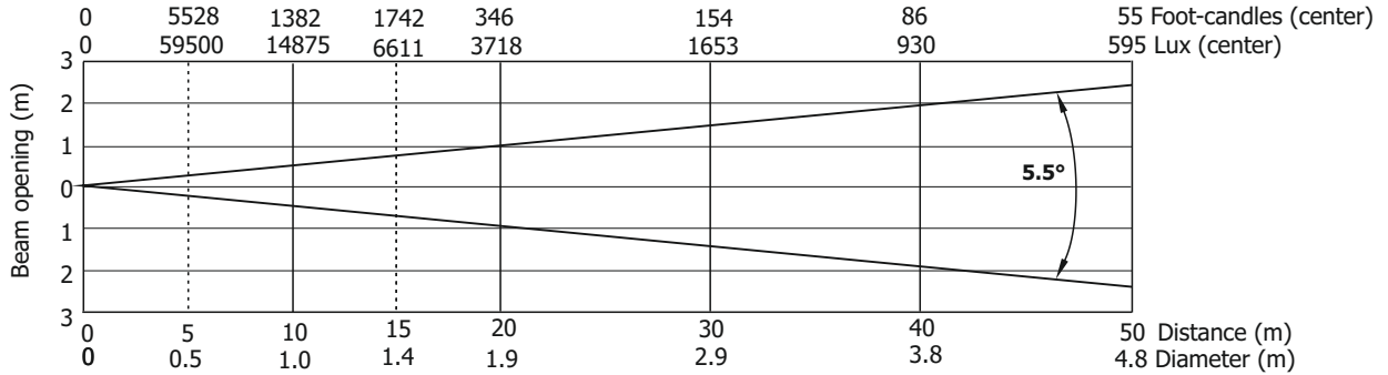
Illuminance distribution
