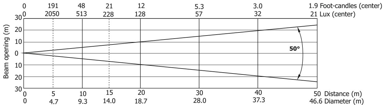
Illuminance distribution
