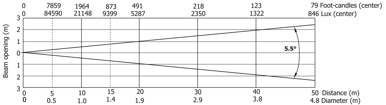
Illuminance distribution
