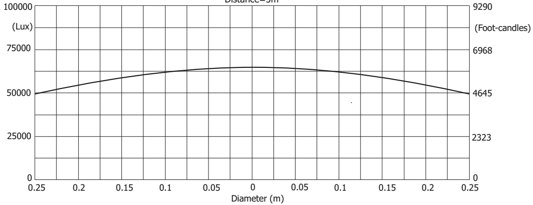
Illuminance distribution
