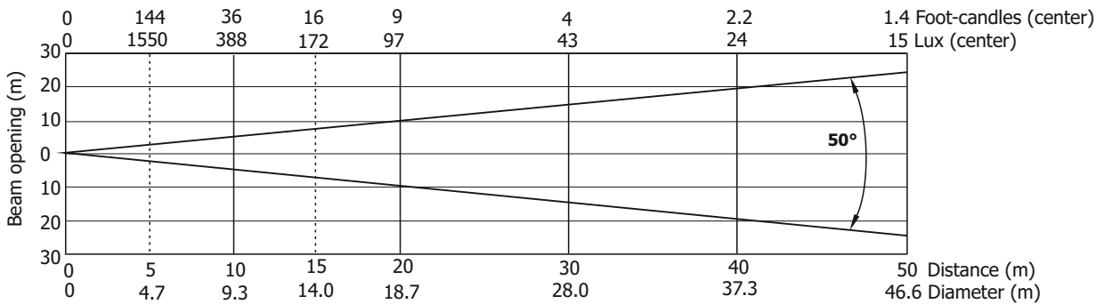
Illuminance distribution
